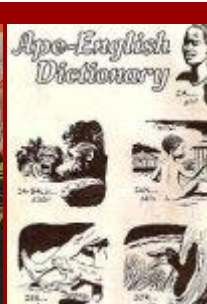
Ape Language
